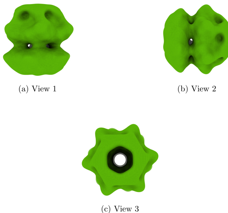
Figure 4: Isosurface at threshold=0.087700. Views generated by ChimeraX at a the following X, Y, Z angles: View 1 (0, -90, -90), View 2 (-90, 0, -90), View 3 (0, 0, 0).
