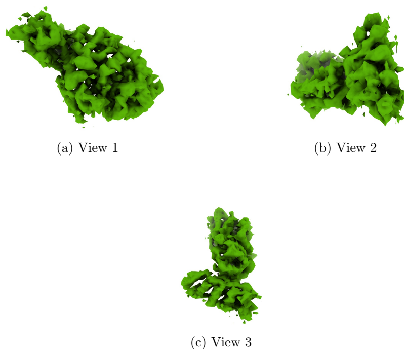
Figure 4: Isosurface at threshold=0.254000. Views generated by ChimeraX at a the following X, Y, Z angles: View 1 (0, -90, -90), View 2 (-90, 0, -90), View 3 (0, 0, 0).
