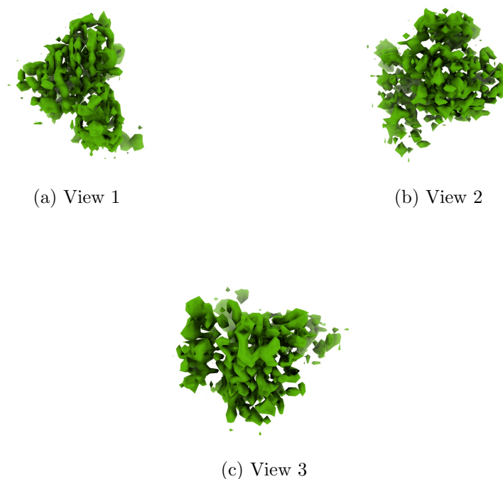
Figure 4: Isosurface at threshold=0.414000. Views generated by ChimeraX at a the following X, Y, Z angles: View 1 (0, -90, -90), View 2 (-90, 0, -90), View 3 (0, 0, 0).
