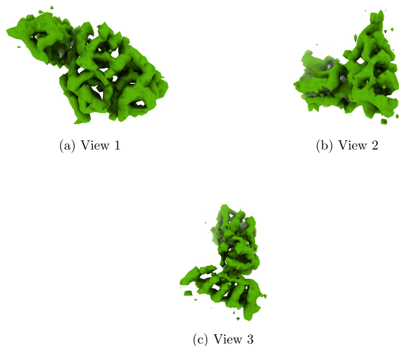
Figure 4: Isosurface at threshold=0.340000. Views generated by ChimeraX at a the following X, Y, Z angles: View 1 (0, -90, -90), View 2 (-90, 0, -90), View 3 (0, 0, 0).
