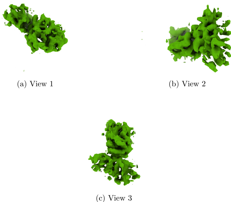
Figure 4: Isosurface at threshold=0.261000. Views generated by ChimeraX at a the following X, Y, Z angles: View 1 (0, -90, -90), View 2 (-90, 0, -90), View 3 (0, 0, 0).
