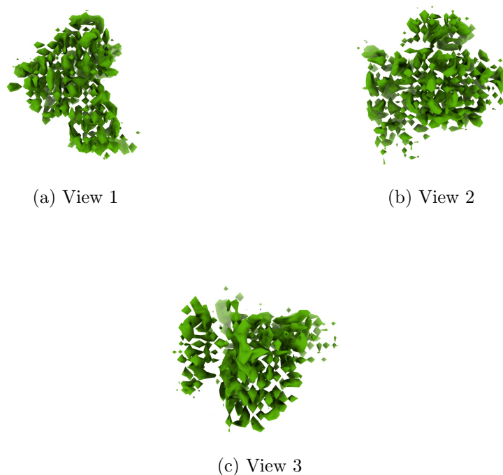
Figure 4: Isosurface at threshold=0.662000. Views generated by ChimeraX at a the following X, Y, Z angles: View 1 (0, -90, -90), View 2 (-90, 0, -90), View 3 (0, 0, 0).
