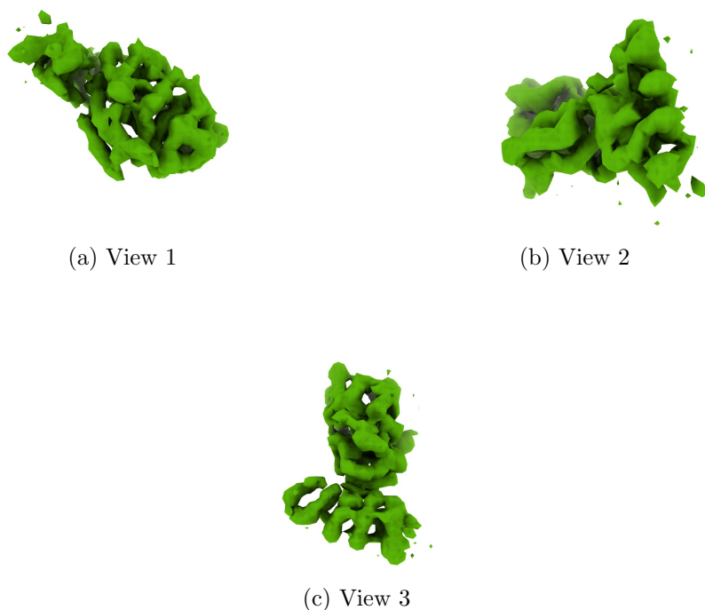
Figure 4: Isosurface at threshold=0.314000. Views generated by ChimeraX at a the following X, Y, Z angles: View 1 (0, -90, -90), View 2 (-90, 0, -90), View 3 (0, 0, 0).
