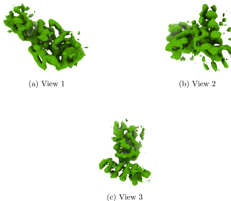
Figure 4: Isosurface at threshold=0.457000. Views generated by ChimeraX at a the following X, Y, Z angles: View 1 (0, -90, -90), View 2 (-90, 0, -90), View 3 (0, 0, 0).
