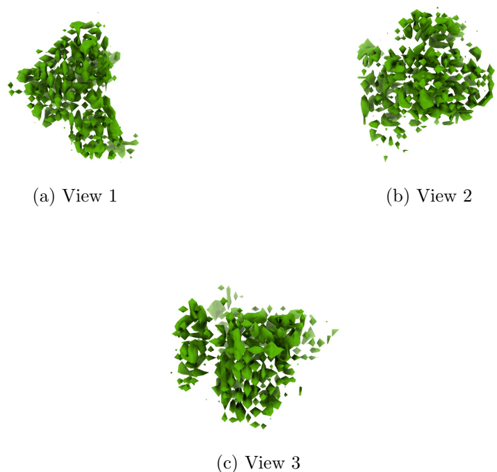
Figure 4: Isosurface at threshold=0.759000. Views generated by ChimeraX at a the following X, Y, Z angles: View 1 (0, -90, -90), View 2 (-90, 0, -90), View 3 (0, 0, 0).
