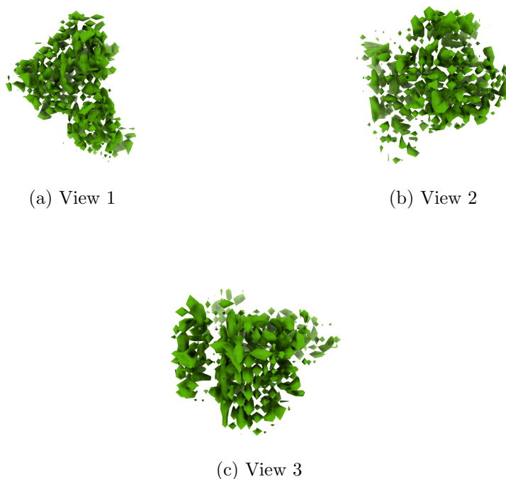
Figure 4: Isosurface at threshold=0.689000. Views generated by ChimeraX at a the following X, Y, Z angles: View 1 (0, -90, -90), View 2 (-90, 0, -90), View 3 (0, 0, 0).
