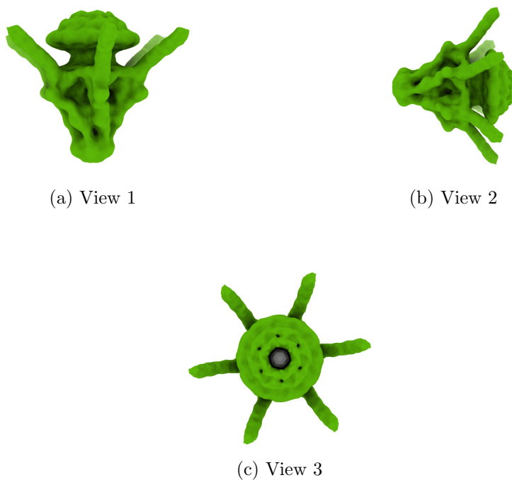
Figure 4: Isosurface at threshold=0.007440. Views generated by ChimeraX at a the following X, Y, Z angles: View 1 (0, -90, -90), View 2 (-90, 0, -90), View 3 (0, 0, 0).
