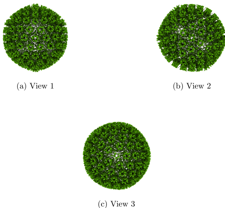
Figure 4: Isosurface at threshold=14.800000. Views generated by ChimeraX at a the following X, Y, Z angles: View 1 (0, -90, -90), View 2 (-90, 0, -90), View 3 (0, 0, 0).
