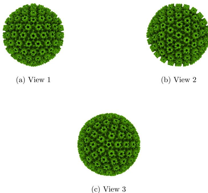
Figure 4: Isosurface at threshold=12.500000. Views generated by ChimeraX at a the following X, Y, Z angles: View 1 (0, -90, -90), View 2 (-90, 0, -90), View 3 (0, 0, 0).
