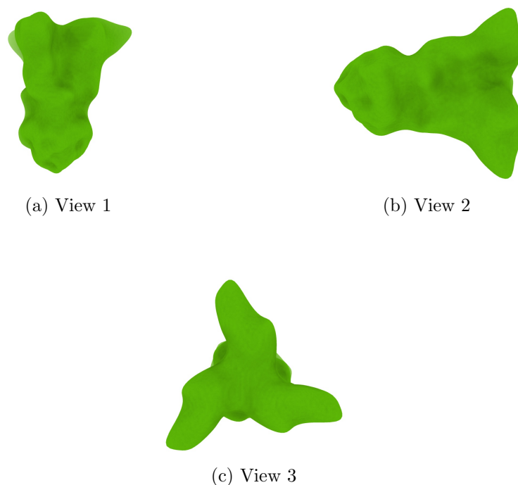
Figure 4: Isosurface at threshold=4.020000. Views generated by ChimeraX at a the following X, Y, Z angles: View 1 (0, -90, -90), View 2 (-90, 0, -90), View 3 (0, 0, 0).
