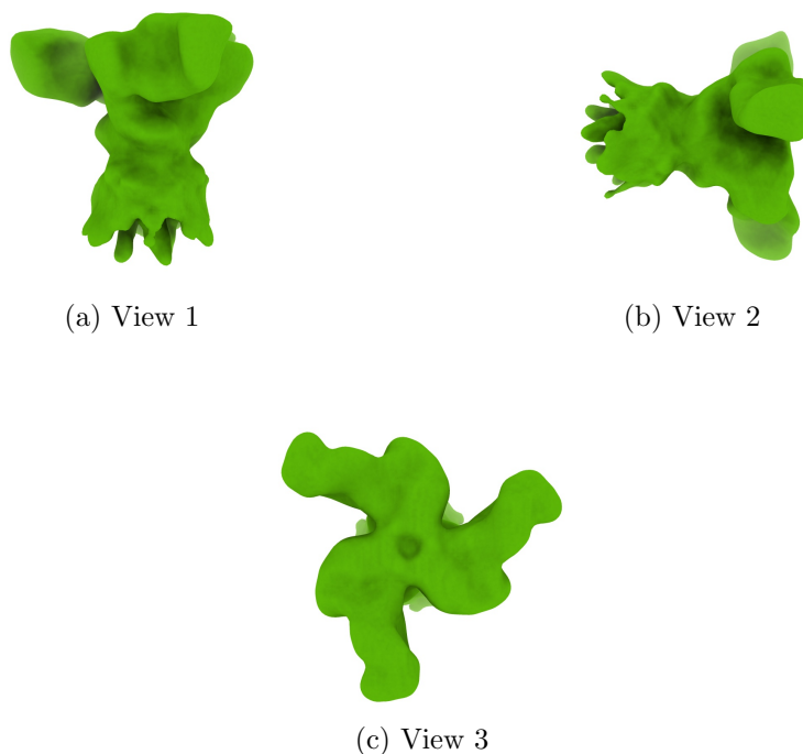
Figure 4: Isosurface at threshold=2.810000. Views generated by ChimeraX at a the following X, Y, Z angles: View 1 (0, -90, -90), View 2 (-90, 0, -90), View 3 (0, 0, 0).
