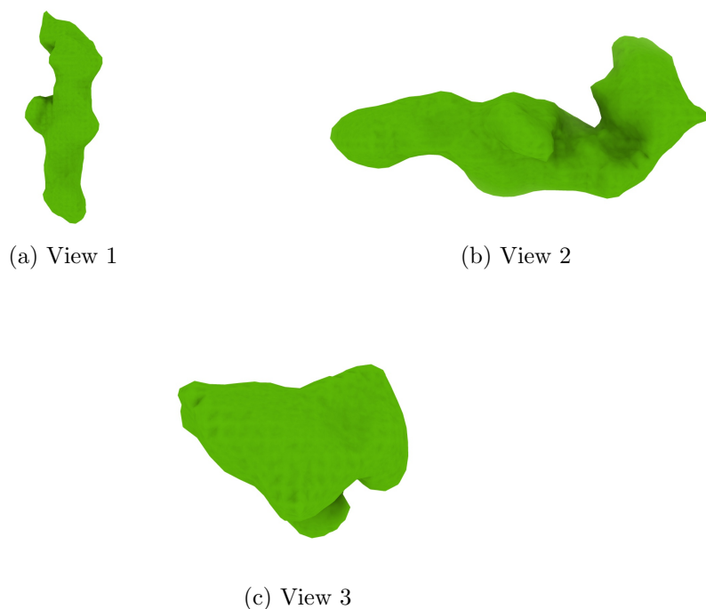
Figure 4: Isosurface at threshold=0.109022. Views generated by ChimeraX at a the following X, Y, Z angles: View 1 (0, -90, -90), View 2 (-90, 0, -90), View 3 (0, 0, 0).
