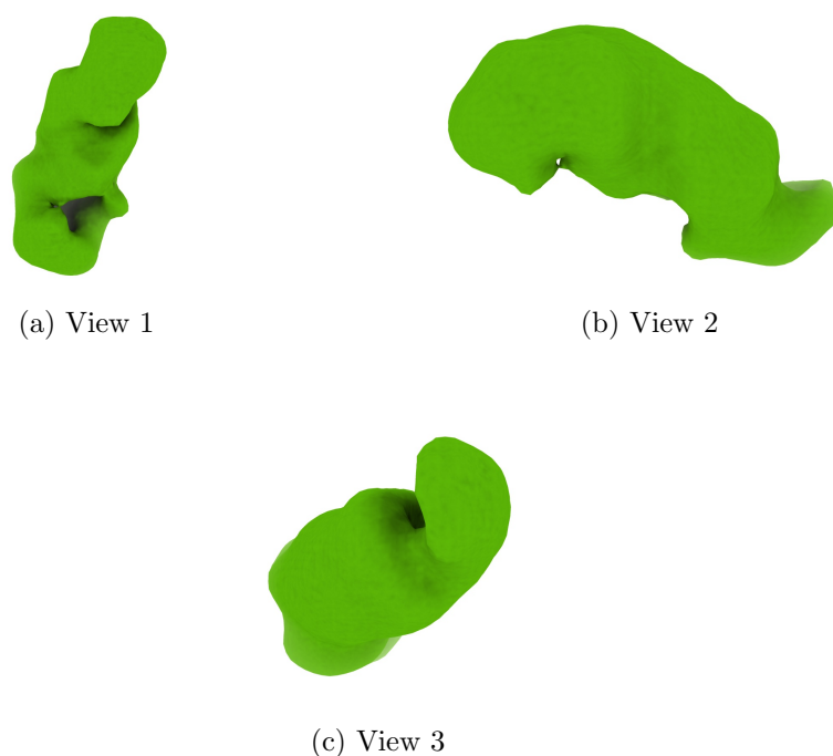
Figure 4: Isosurface at threshold=0.620000. Views generated by ChimeraX at the following X, Y, Z angles: View 1 (0, -90, -90), View 2 (-90, 0, -90), View 3 (0, 0, 0).
