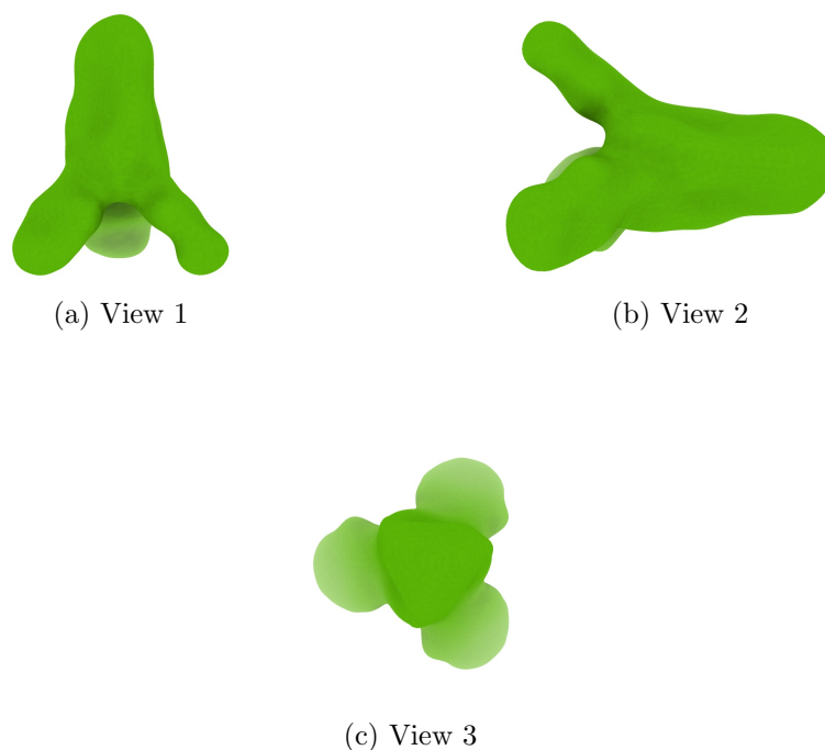
Figure 4: Isosurface at threshold=3.020000. Views generated by ChimeraX at a the following X, Y, Z angles: View 1 (0, -90, -90), View 2 (-90, 0, -90), View 3 (0, 0, 0).
