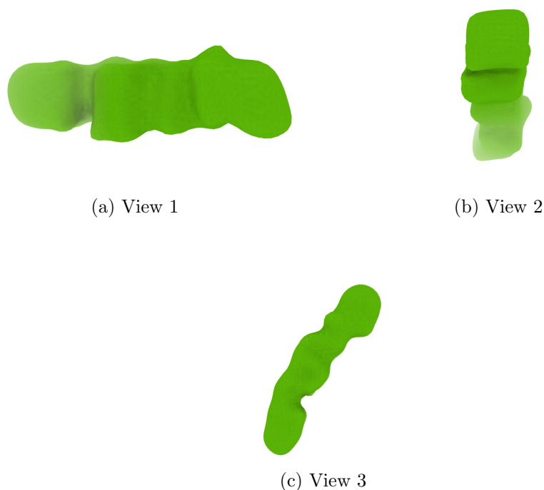
Figure 4: Isosurface at threshold=0.507000. Views generated by ChimeraX at a the following X, Y, Z angles: View 1 (0, -90, -90), View 2 (-90, 0, -90), View 3 (0, 0, 0).
