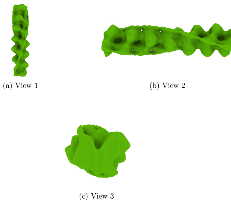
Figure 4: Isosurface at threshold=0.453000. Views generated by ChimeraX at a the following X, Y, Z angles: View 1 (0, -90, -90), View 2 (-90, 0, -90), View 3 (0, 0, 0).
