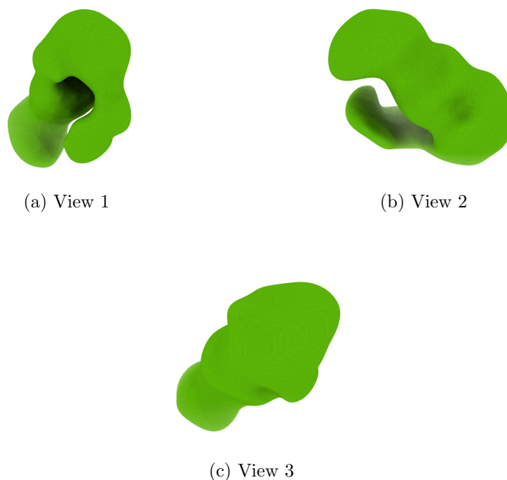
Figure 4: Isosurface at threshold=1.720000. Views generated by ChimeraX at a the following X, Y, Z angles: View 1 (0, -90, -90), View 2 (-90, 0, -90), View 3 (0, 0, 0).
