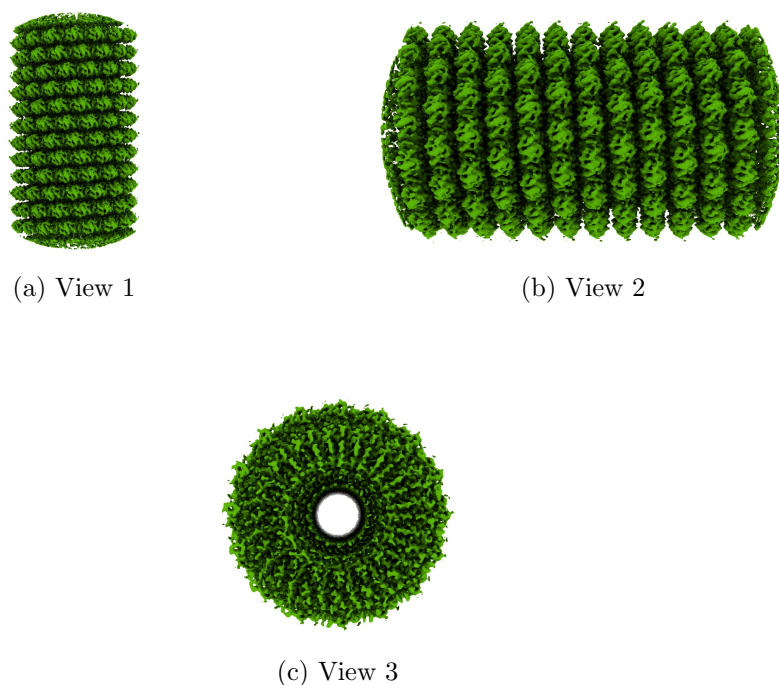
Figure 4: Isosurface at threshold=0.008000. Views generated by ChimeraX at the following X, Y, Z angles: View 1 (0, -90, -90), View 2 (-90, 0, -90), View 3 (0, 0, 0).
