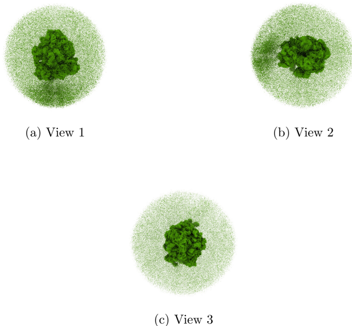
Figure 4: Isosurface at threshold=0.103000. Views generated by ChimeraX at a the following X, Y, Z angles: View 1 (0, -90, -90), View 2 (-90, 0, -90), View 3 (0, 0, 0).
