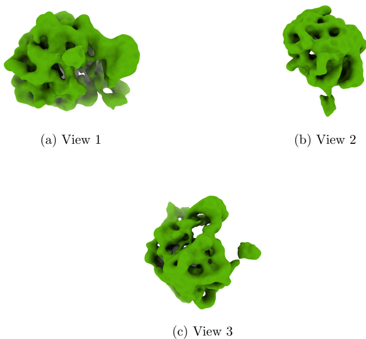
Figure 4: Isosurface at threshold=2.540000. Views generated by ChimeraX at a the following X, Y, Z angles: View 1 (0, -90, -90), View 2 (-90, 0, -90), View 3 (0, 0, 0).
