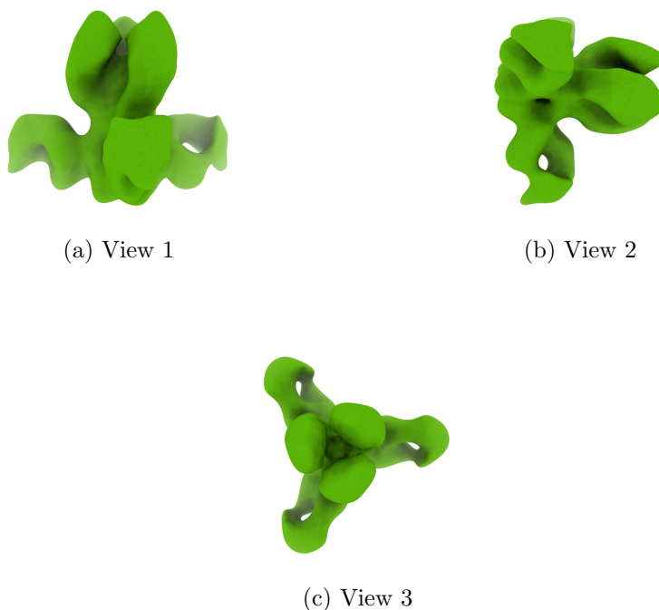
Figure 4: Isosurface at threshold=8.080000. Views generated by ChimeraX at a the following X, Y, Z angles: View 1 (0, -90, -90), View 2 (-90, 0, -90), View 3 (0, 0, 0).
