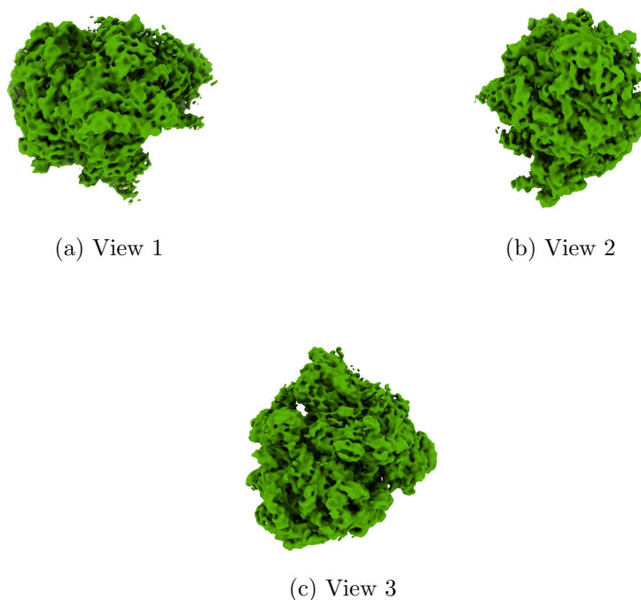
Figure 4: Isosurface at threshold=0.340000. Views generated by ChimeraX at a the following X, Y, Z angles: View 1 (0, -90, -90), View 2 (-90, 0, -90), View 3 (0, 0, 0).
