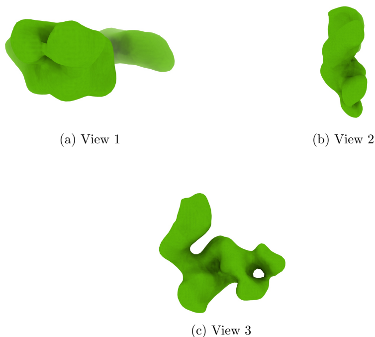
Figure 4: Isosurface at threshold=0.022600. Views generated by ChimeraX at a the following X, Y, Z angles: View 1 (0, -90, -90), View 2 (-90, 0, -90), View 3 (0, 0, 0).
