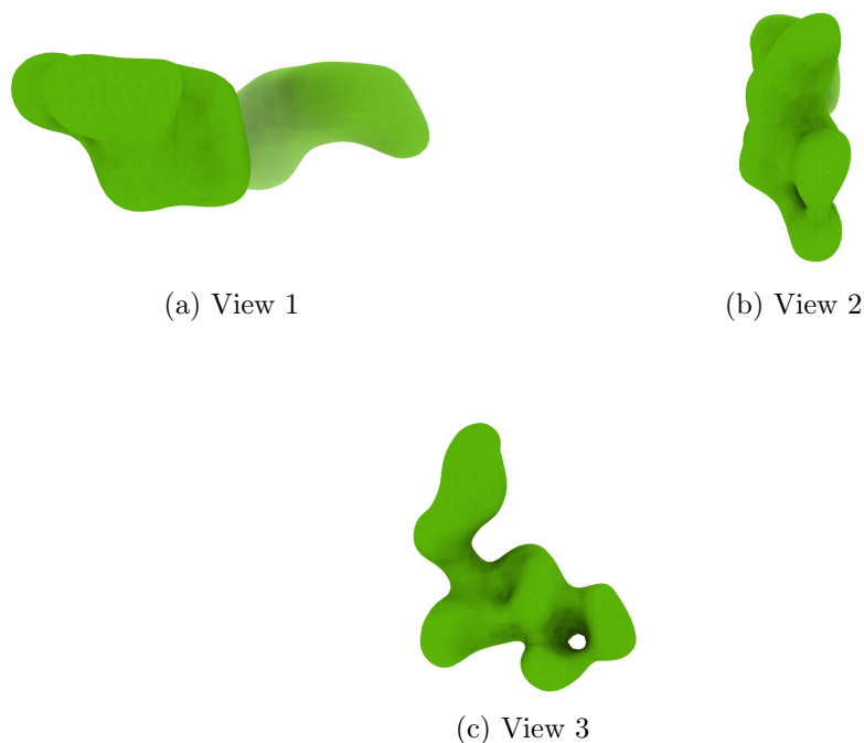
Figure 4: Isosurface at threshold=0.020500. Views generated by ChimeraX at a the following X, Y, Z angles: View 1 (0, -90, -90), View 2 (-90, 0, -90), View 3 (0, 0, 0).
