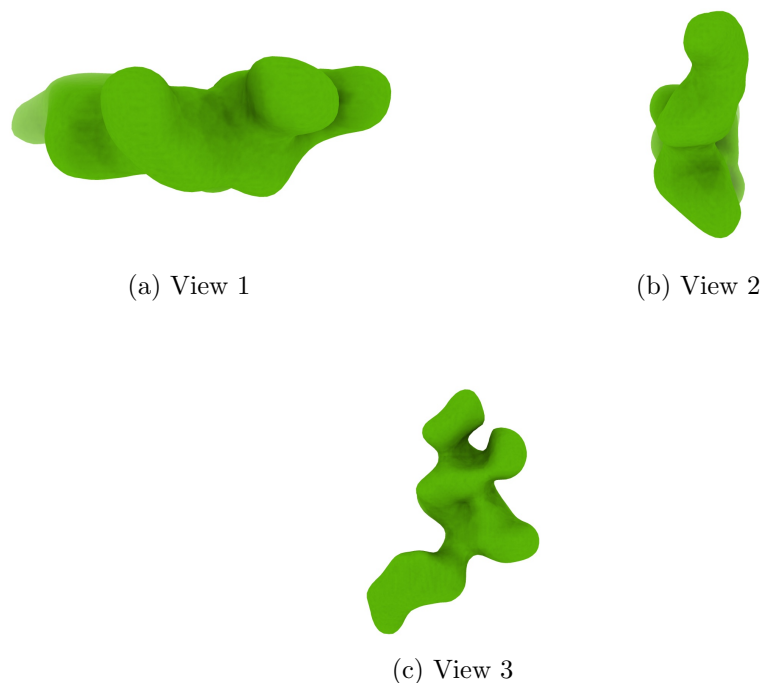
Figure 4: Isosurface at threshold=0.021400. Views generated by ChimeraX at a the following X, Y, Z angles: View 1 (0, -90, -90), View 2 (-90, 0, -90), View 3 (0, 0, 0).
