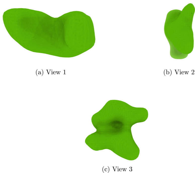
Figure 4: Isosurface at threshold=0.020300. Views generated by ChimeraX at a the following X, Y, Z angles: View 1 (0, -90, -90), View 2 (-90, 0, -90), View 3 (0, 0, 0).
