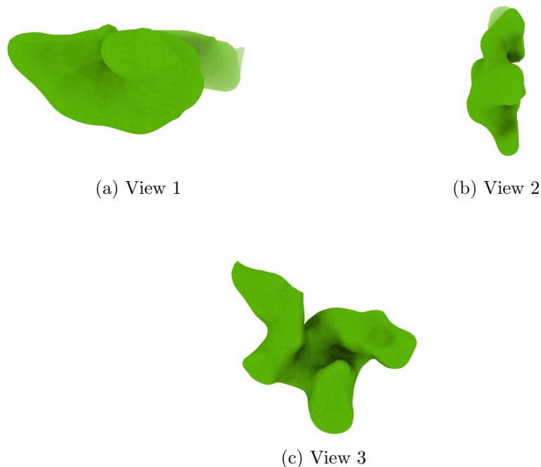
Figure 4: Isosurface at threshold=0.030800. Views generated by ChimeraX at a the following X, Y, Z angles: View 1 (0, -90, -90), View 2 (-90, 0, -90), View 3 (0, 0, 0).
