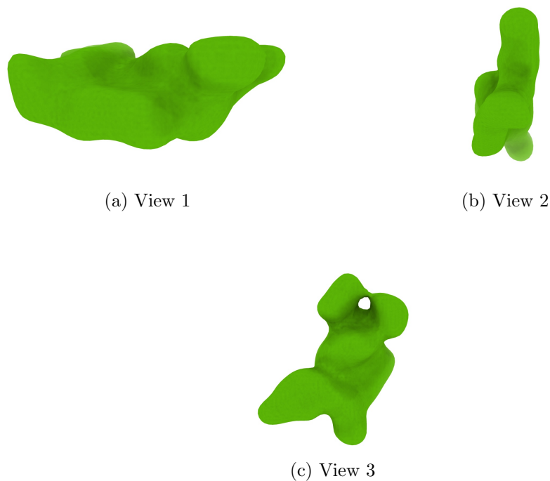
Figure 4: Isosurface at threshold=0.024700. Views generated by ChimeraX at the following X, Y, Z angles: View 1 (0, -90, -90), View 2 (-90, 0, -90), View 3 (0, 0, 0).
