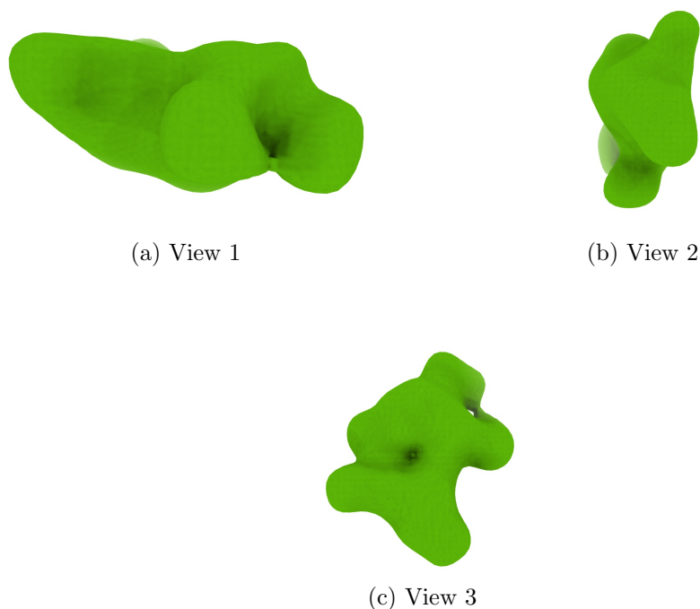
Figure 4: Isosurface at threshold=0.023400. Views generated by ChimeraX at a the following X, Y, Z angles: View 1 (0, -90, -90), View 2 (-90, 0, -90), View 3 (0, 0, 0).
