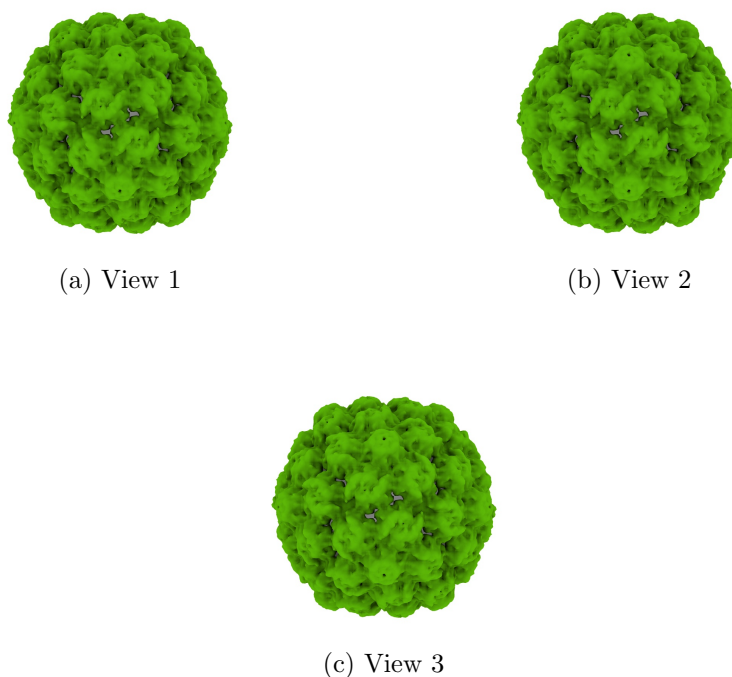
Figure 4: Isosurface at threshold=0.082600. Views generated by ChimeraX at a the following X, Y, Z angles: View 1 (0, -90, -90), View 2 (-90, 0, -90), View 3 (0, 0, 0).
