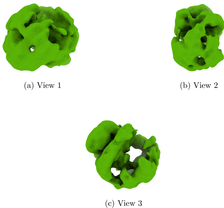
Figure 4: Isosurface at threshold=0.438000. Views generated by ChimeraX at a the following X, Y, Z angles: View 1 (0, -90, -90), View 2 (-90, 0, -90), View 3 (0, 0, 0).
