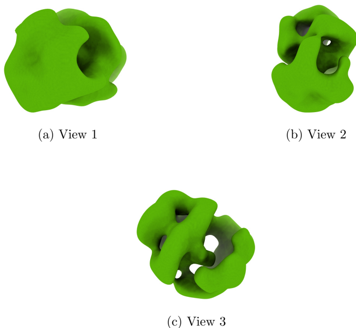
Figure 4: Isosurface at threshold=0.029400. Views generated by ChimeraX at a the following X, Y, Z angles: View 1 (0, -90, -90), View 2 (-90, 0, -90), View 3 (0, 0, 0).
