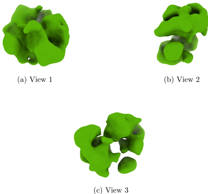
Figure 4: Isosurface at threshold=5.390000. Views generated by ChimeraX at a the following X, Y, Z angles: View 1 (0, -90, -90), View 2 (-90, 0, -90), View 3 (0, 0, 0).
