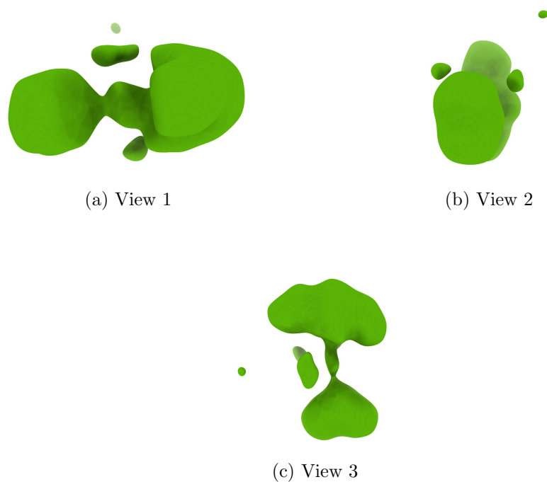
Figure 4: Isosurface at threshold=0.628000. Views generated by ChimeraX at a the following X, Y, Z angles: View 1 (0, -90, -90), View 2 (-90, 0, -90), View 3 (0, 0, 0).
