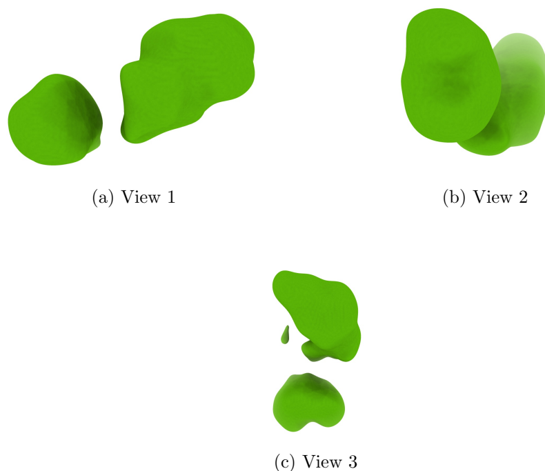
Figure 4: Isosurface at threshold=0.802000. Views generated by ChimeraX at a the following X, Y, Z angles: View 1 (0, -90, -90), View 2 (-90, 0, -90), View 3 (0, 0, 0).
