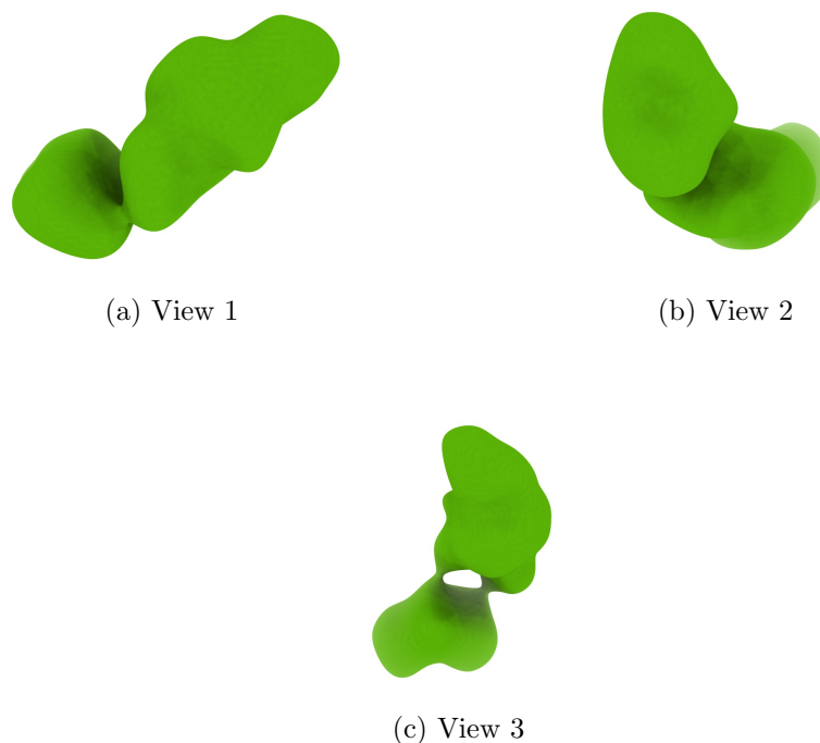
Figure 4: Isosurface at threshold=0.968000. Views generated by ChimeraX at a the following X, Y, Z angles: View 1 (0, -90, -90), View 2 (-90, 0, -90), View 3 (0, 0, 0).
