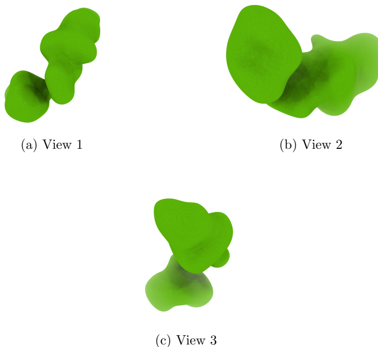
Figure 4: Isosurface at threshold=0.992000. Views generated by ChimeraX at a the following X, Y, Z angles: View 1 (0, -90, -90), View 2 (-90, 0, -90), View 3 (0, 0, 0).
