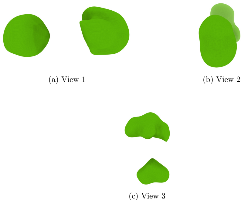
Figure 4: Isosurface at threshold=1.130000. Views generated by ChimeraX at the following X, Y, Z angles: View 1 (0, -90, -90), View 2 (-90, 0, -90), View 3 (0, 0, 0).
