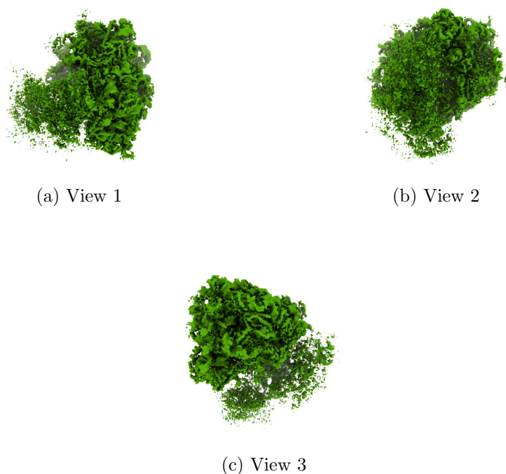
Figure 4: Isosurface at threshold=8.750000. Views generated by ChimeraX at a the following X, Y, Z angles: View 1 (0, -90, -90), View 2 (-90, 0, -90), View 3 (0, 0, 0).
