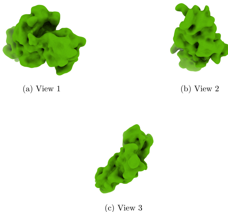
Figure 4: Isosurface at threshold=2.750000. Views generated by ChimeraX at a the following X, Y, Z angles: View 1 (0, -90, -90), View 2 (-90, 0, -90), View 3 (0, 0, 0).
