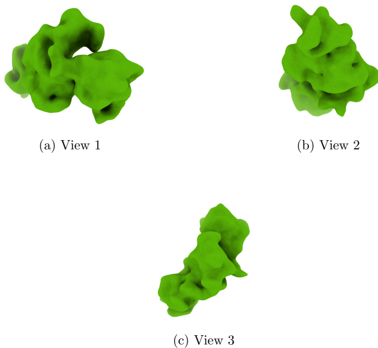
Figure 4: Isosurface at threshold=2.840000. Views generated by ChimeraX at a the following X, Y, Z angles: View 1 (0, -90, -90), View 2 (-90, 0, -90), View 3 (0, 0, 0).
