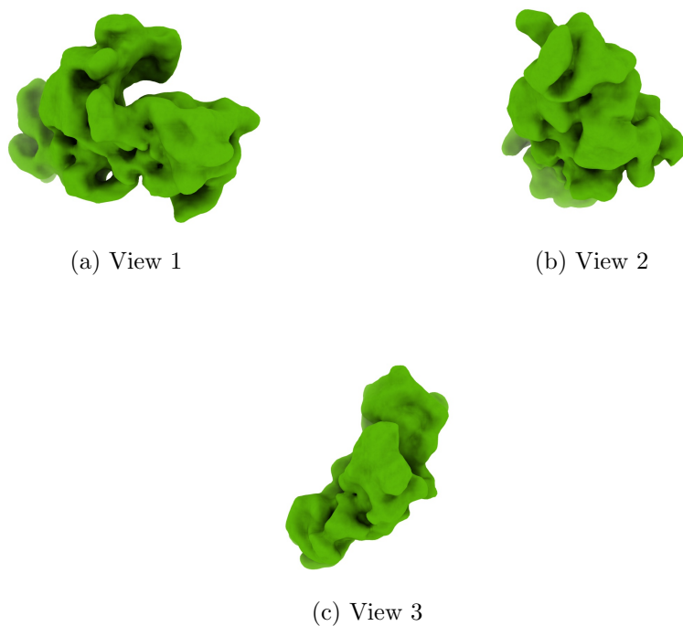
Figure 4: Isosurface at threshold=2.960000. Views generated by ChimeraX at a the following X, Y, Z angles: View 1 (0, -90, -90), View 2 (-90, 0, -90), View 3 (0, 0, 0).
