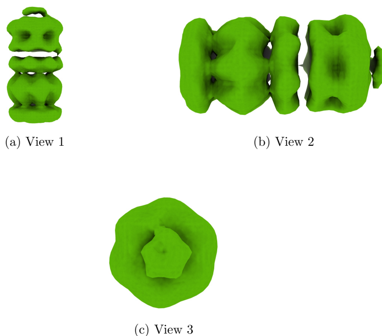
Figure 4: Isosurface at threshold=2.000000. Views generated by ChimeraX at a the following X, Y, Z angles: View 1 (0, -90, -90), View 2 (-90, 0, -90), View 3 (0, 0, 0).
