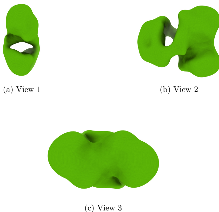
Figure 4: Isosurface at threshold=0.149000. Views generated by ChimeraX at a the following X, Y, Z angles: View 1 (0, -90, -90), View 2 (-90, 0, -90), View 3 (0, 0, 0).
