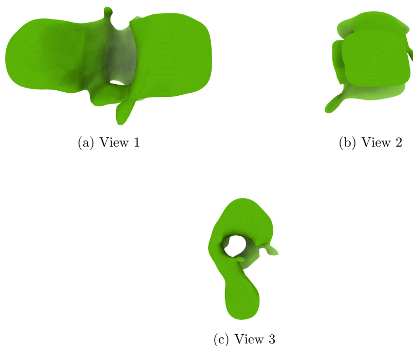
Figure 4: Isosurface at threshold=0.537000. Views generated by ChimeraX at a the following X, Y, Z angles: View 1 (0, -90, -90), View 2 (-90, 0, -90), View 3 (0, 0, 0).
