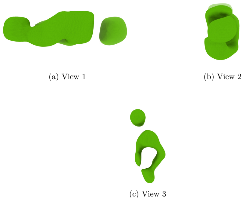
Figure 4: Isosurface at threshold=0.650000. Views generated by ChimeraX at a the following X, Y, Z angles: View 1 (0, -90, -90), View 2 (-90, 0, -90), View 3 (0, 0, 0).
